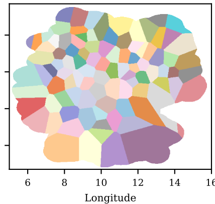
(c) Wind weather aggregation 100 clusters, wind-capacity weights
